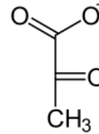
Pyruvate
