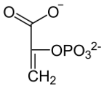
Phosphoenolpyruvate
