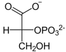
Glycerate 2 phosphate
