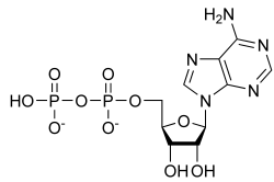
ADP
